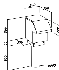
SEM 5 remote motor for outdoor price € 822,00
