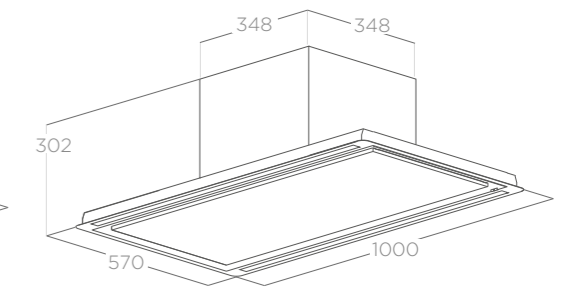
FALSE CEILING CUT 550X980
