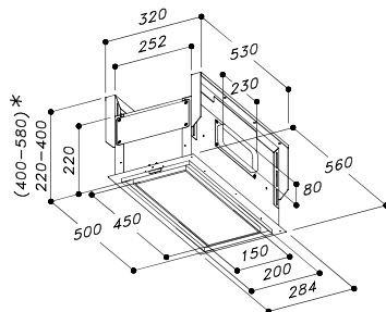
S-DF2** AIR DEVIATOR FOR USE WITH CEILING HOODS WHEN RECIRCULATING BUILT-IN VERSION The air deviator needs to be installed at a minimum distance of 1500mm from the extractor
