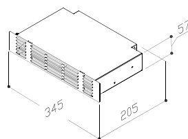
S-KFHE3 HIGH EFFICIENCY FILTERING KIT FOR KITCHEN PLINT MIN. 60mm HEIGHT
